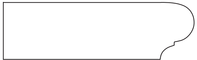
WINDOW STOOL AVAILABLE IN 3 WIDTHS 1-1/16" x 2-1/2" 1-1/16" x 3-1/2" 1-1/16" x 5-1/2" #PB903
